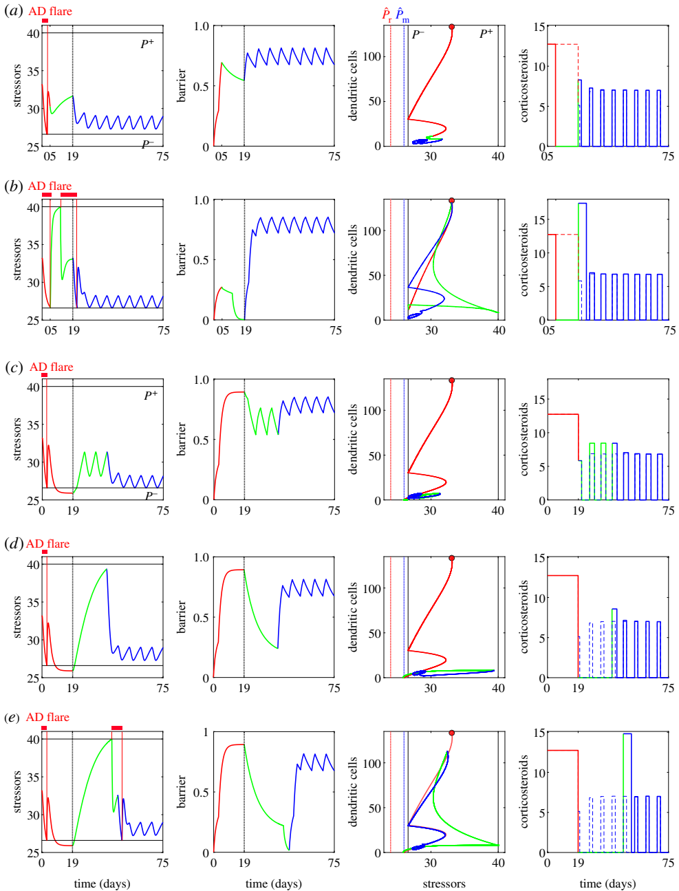
Figure 5. Effects of poor adherence to the calculated optimal treatment strategies. Non-adherence to the suggested corticosteroid treatment after 5 days in the induction phase, with continual use of emollients ( a ) and without use of emollients ( b ). Non-adherence to the suggested corticosteroid treatment during the maintenance phase, without emollient application for the first three cycles ( c ), and without both corticosteroid and emollient application for the first three cycles ( d ) and four cycles ( e ). Green lines represent the period during the non-adherence, and the dotted lines on the right column demonstrate the optimal strategy calculated for the nominal case where patients adhere to the suggested optimal strategy.
