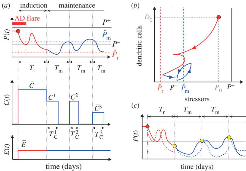
Figure 2. Optimal control problem formulation to design treatment strategies for proactive therapy for AD. The whole period consists of the induction phase (red) and maintenance phase (blue). (a) An example dynamics of a state variable ( P(t) ) with on–off treatment of corticosteroids ( C(t) ) of different potencies at discrete times, in addition to constant application of emollients ( E(t) ) of a fixed potency \bar{E} . (b) An example trajectory of a projection of a patient's states, ( P, D ), when the optimal treatment strategy is applied. The states move from the initial state ( (P_0, D_0) , red circle) towards the target level, \hat{P}_r , of the induction phase (red vertical line), and then to the target level, \hat{P}_m , of the maintenance phase (blue vertical line). The state B is omitted in the figure. (c) The recursive optimal control problem to be solved. The optimal treatment strategy for each cycle (either for the duration of T_r or T_m ) is determined by predicting the optimal evolution of the state variables (dashed lines) based on the measurement of the states at the beginning of the period (circles). The actual evolution of the state (solid lines) can be different from the prediction, for example if the calculated optimal treatment strategy is not applied.
