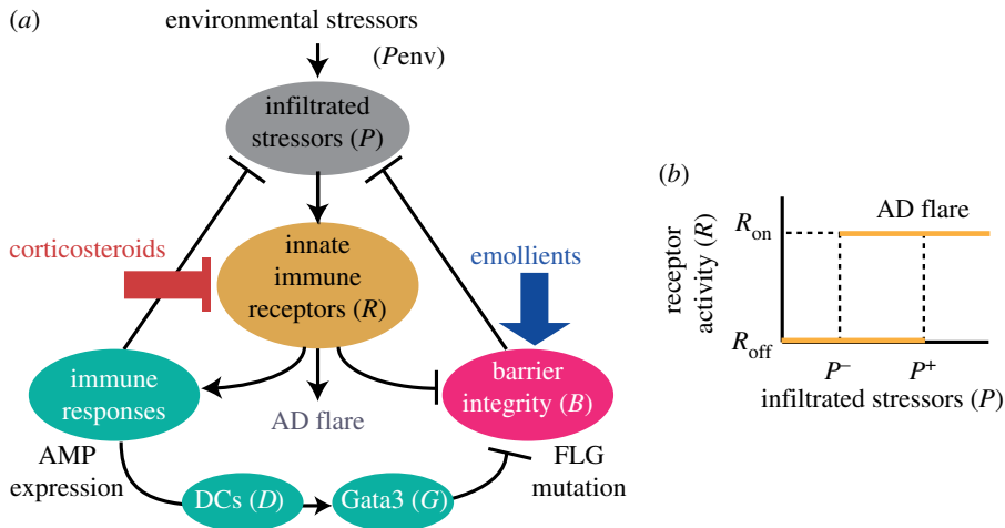
Figure 1. Mathematical model of treatment effects on AD pathogenesis. (a) A model schematic and (b) a perfect reversible switch for the AD flare triggered by infiltrated pathogens. The italics denote the model variables.
