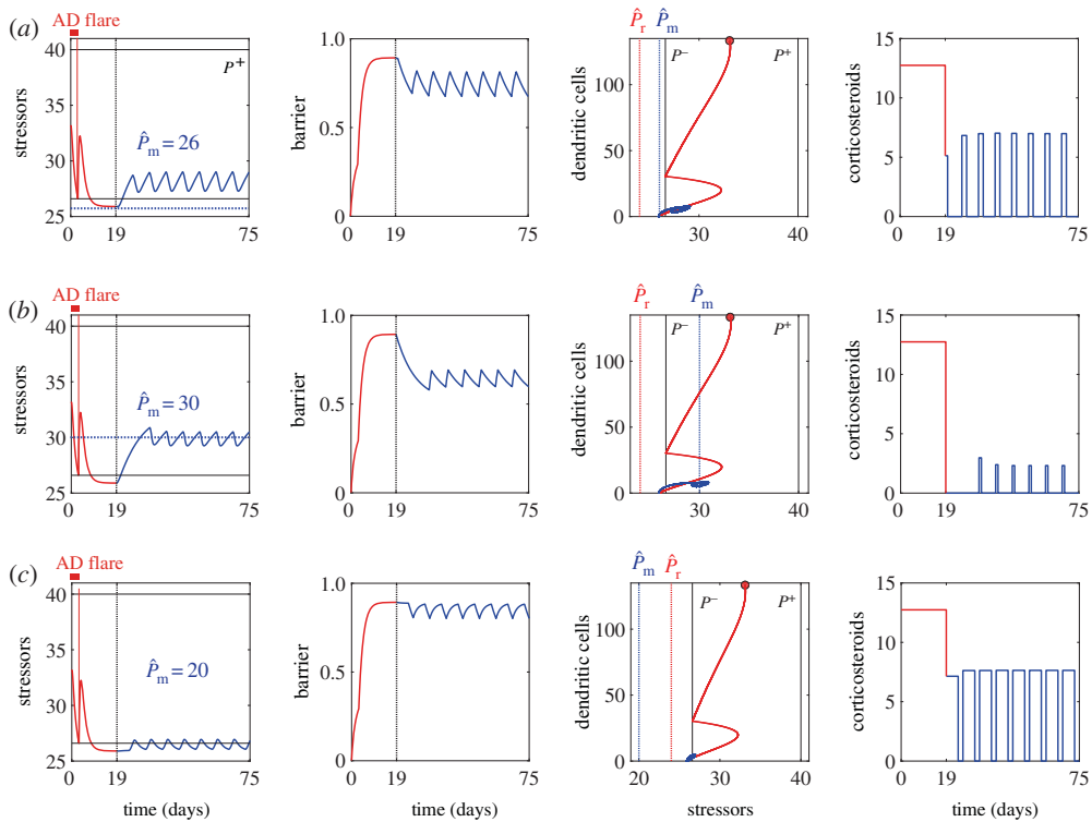
Figure 3. Effects of the choice of the maintenance target level (blue dotted lines) on the optimal treatment strategies calculated and the resulting dynamics of the system. The maintenance target level is set to be (a) \hat{P}_m = 26 (the nominal value), (b) \hat{P}_m = 30 and (c) \hat{P}_m = 20 , while the induction target level (red vertical lines) is set to be the same ( \hat{P}_r = 24 ) for all the scenarios. The dynamics during the induction phase and that during the maintenance phase are shown in red and blue, respectively. Remission is achieved when the level of the stressors is decreased below P^- , and the AD flare reoccurs when it increases above P^+ . The induction phase continues even after the AD flare ceases, and tries to bring the state towards the target level.
