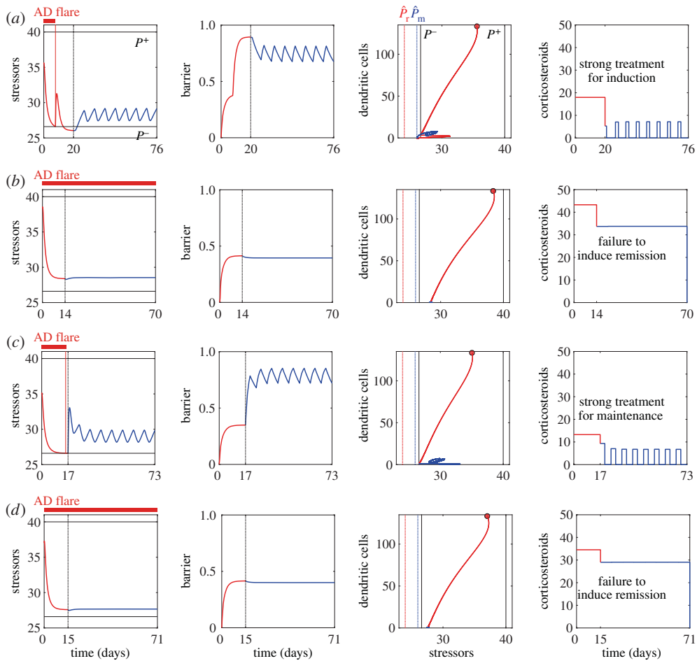
Figure 4. Calculated optimal treatment strategies for different patient cohorts with dysfunctional immune responses: (a) (\kappa_P, \alpha_I) = (0.85, 0.04) and (b) (\kappa_P, \alpha_I) = (0.85, 0.03) ; and compromised barrier integrity: (c) (\kappa_P, \alpha_I) = (0.9, 0.05) and (d) (\kappa_P, \alpha_I) = (0.95, 0.05) . The dynamics during the induction phase starting from the initial state (red circles) is shown in red, and that for the maintenance phase is in blue.
